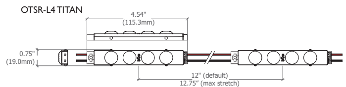
4-bulb, Large body, 1 modules per ft
