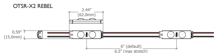
2-bulb, Small body, 2 modules per ft
